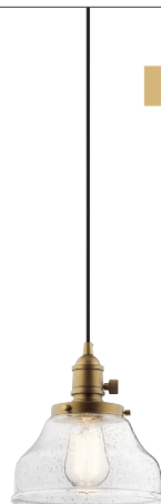
43850NBR | Avery (1) 100W, Medium, 8"W x 8.5"H Overall Ht. 125"
